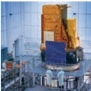
INTEGRAL satellite during vibration test
