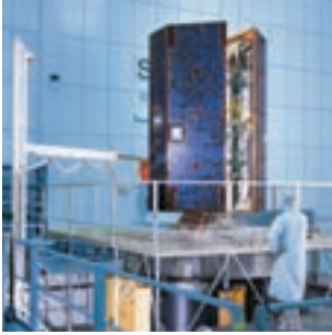
GRACE satellites on the 300 kN shaker
