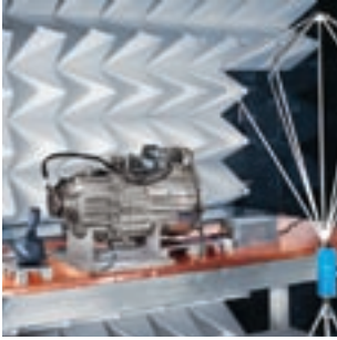
Gear unit in the EMC chamber
