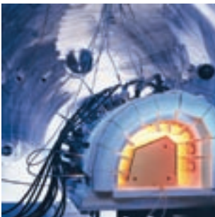
High temperature test on the X-38 wing leading edge
