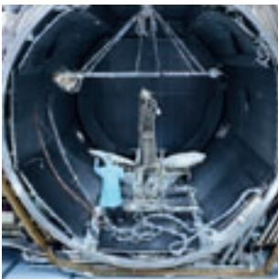
Thermal distortion test on the AMAZONAS top floor antenna
